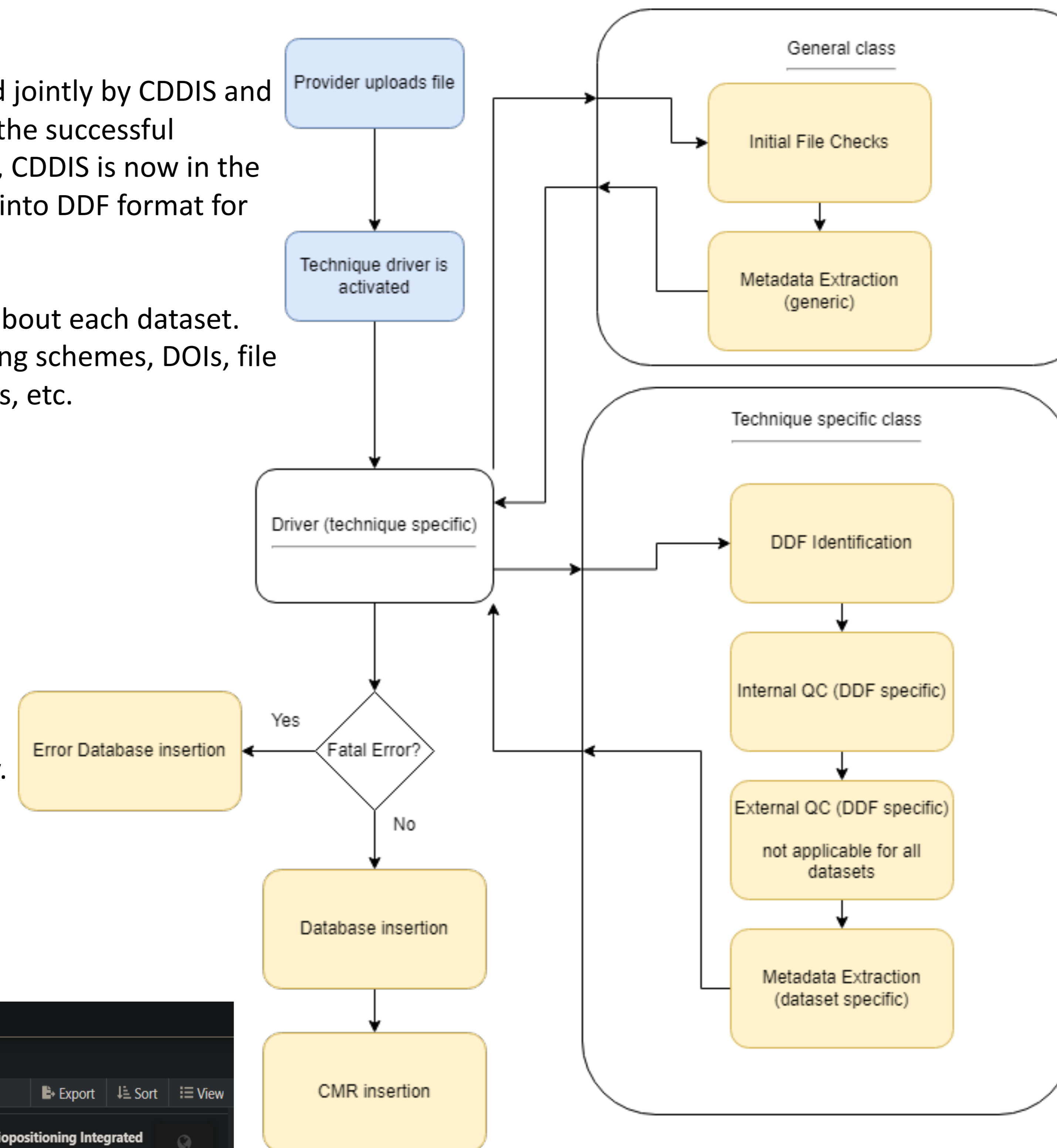
Figure 2. CDDIS Ingest Architecture using DDFs
